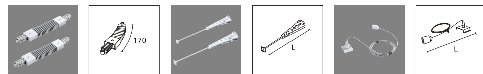
HT-J05 Flexible connector 230V · 16A HT-J06 Pendant crutch Length: 200-1000mm HT-J09 Pendant cable Max load: 100N Length: 3000mm
